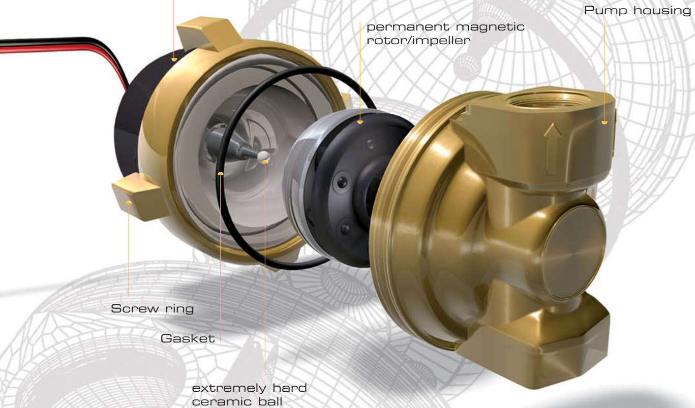
Stator / Pump motor with red speed controller in the end cap
